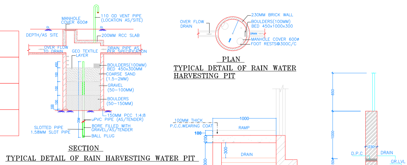
TYPICAL DETAIL OF RAIN HARVESTING WATER PIT
